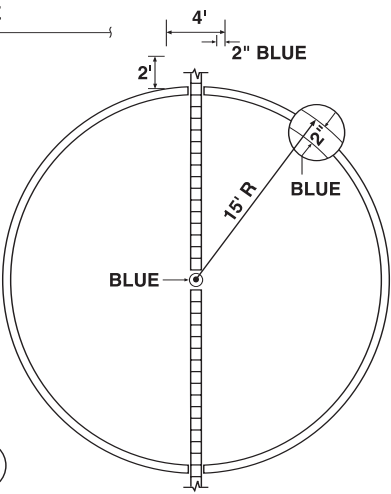
CENTER ICE FACE-OFF SPOT 12" DIA. COLOR BLUE
